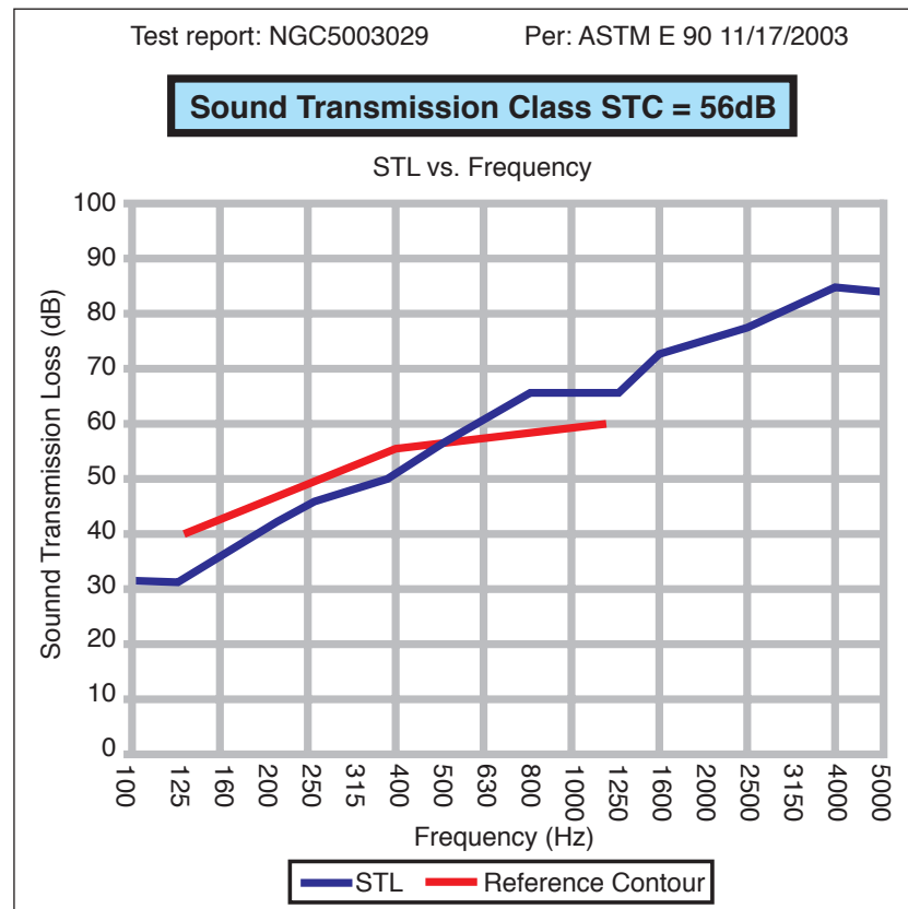
Sound Transmission Loss data for Hardwood Oak Finish/Underlay/Plywood Subfloor over 3mm Acoustiblok, STC 56 See illustration and description on previous page for details of the assembly.
