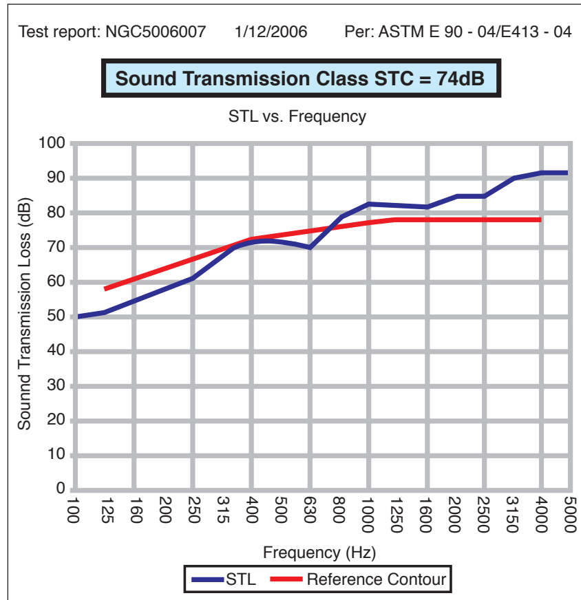
Sound Transmission Loss data for 150mm reinforced concrete slab floor with quarry tile, 16oz Acoustiblok, and gypsum board drop ceiling, STC 74 rated.
