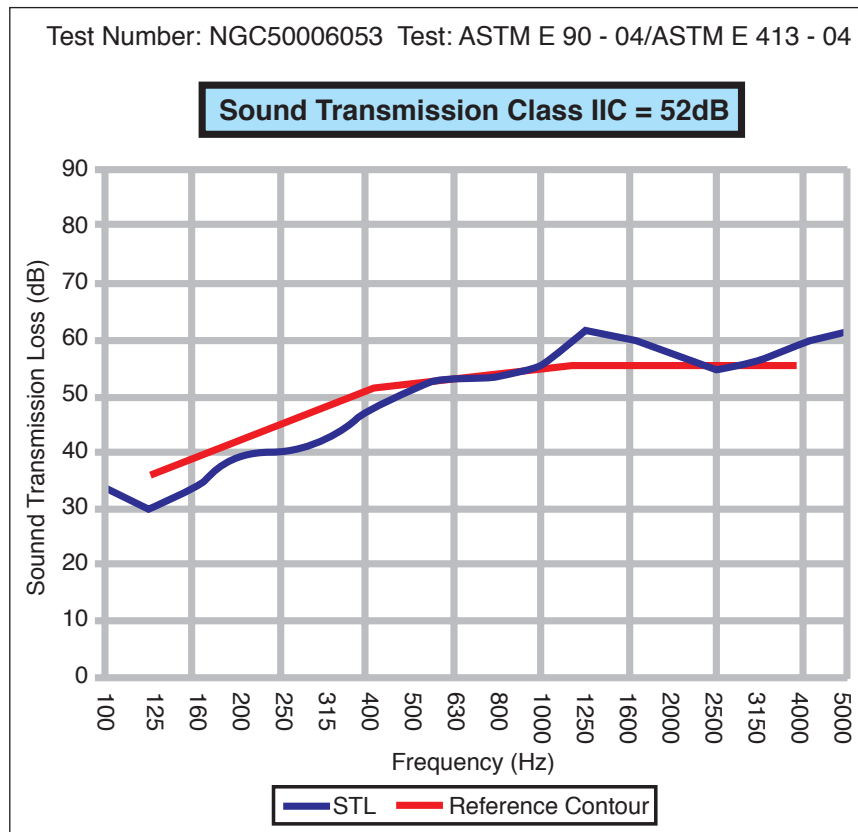
Sound Transmission Loss data for concrete & steel floor/ceiling assembly with 16oz Acoustiblok, STC 52. See illustration and description on previous page for details of the assembly.
